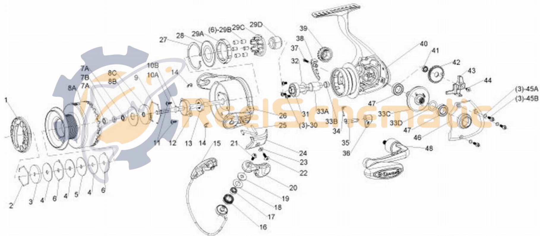
BOCA CABO SERVICE PARTS DIAGRAM
